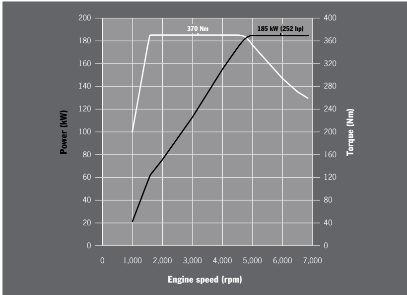
Macan: 370 Nm at 1,600–4,500 rpm, 185 kW (252 hp) at 5,000–6,800 rpm
